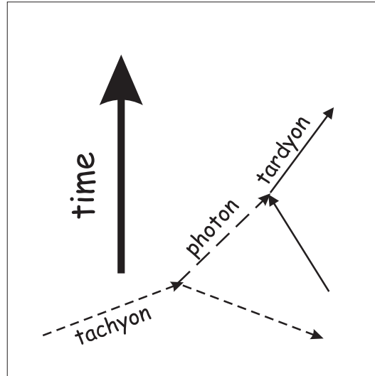
Fig. 6. A tachyon-tachyon interaction using a photon.
